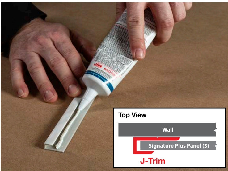
Apply adhesive into J-trim piece.
