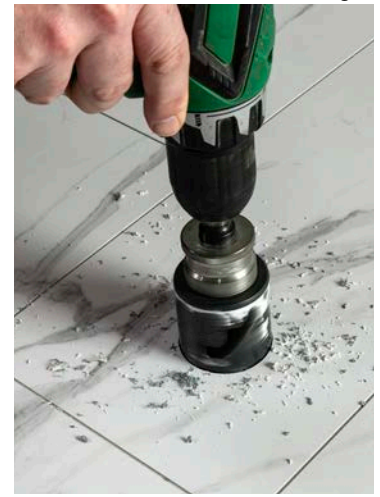
Cut panels to accommodate shower components. Measure and mark the locations and use one of these types of drills or hole saws.
